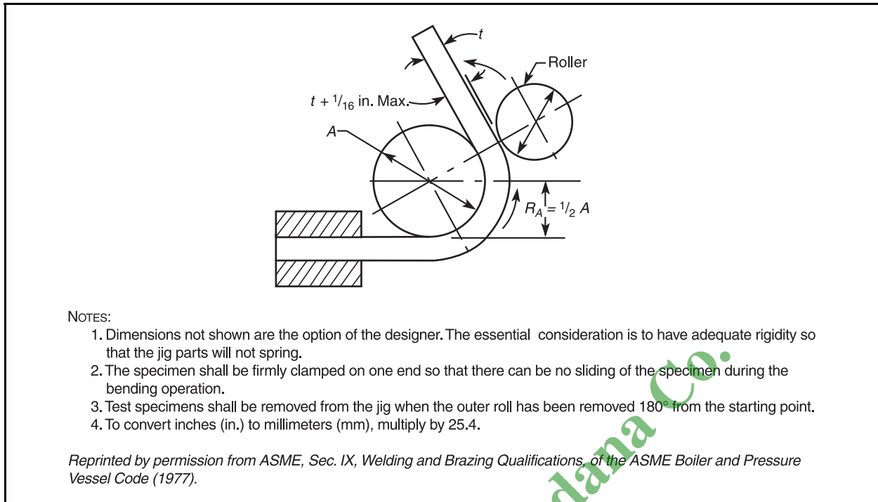
Figure 4 Alternative guided-bend wraparound jig
