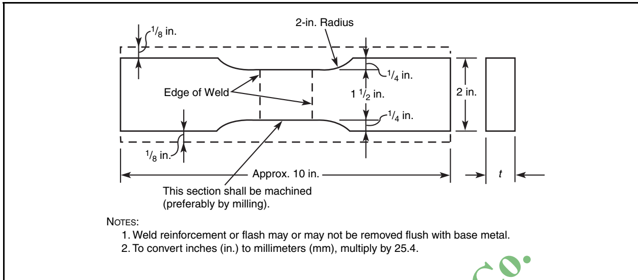
Figure 1 Reduced-section tension test specimen
