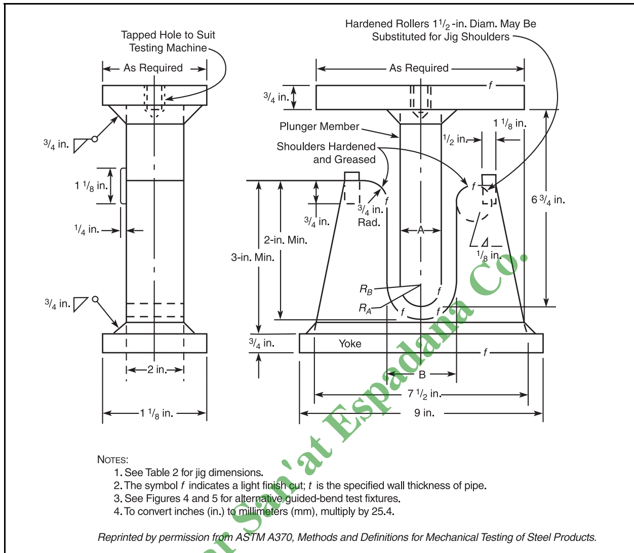
Figure 3 Jig for guided-bend test
