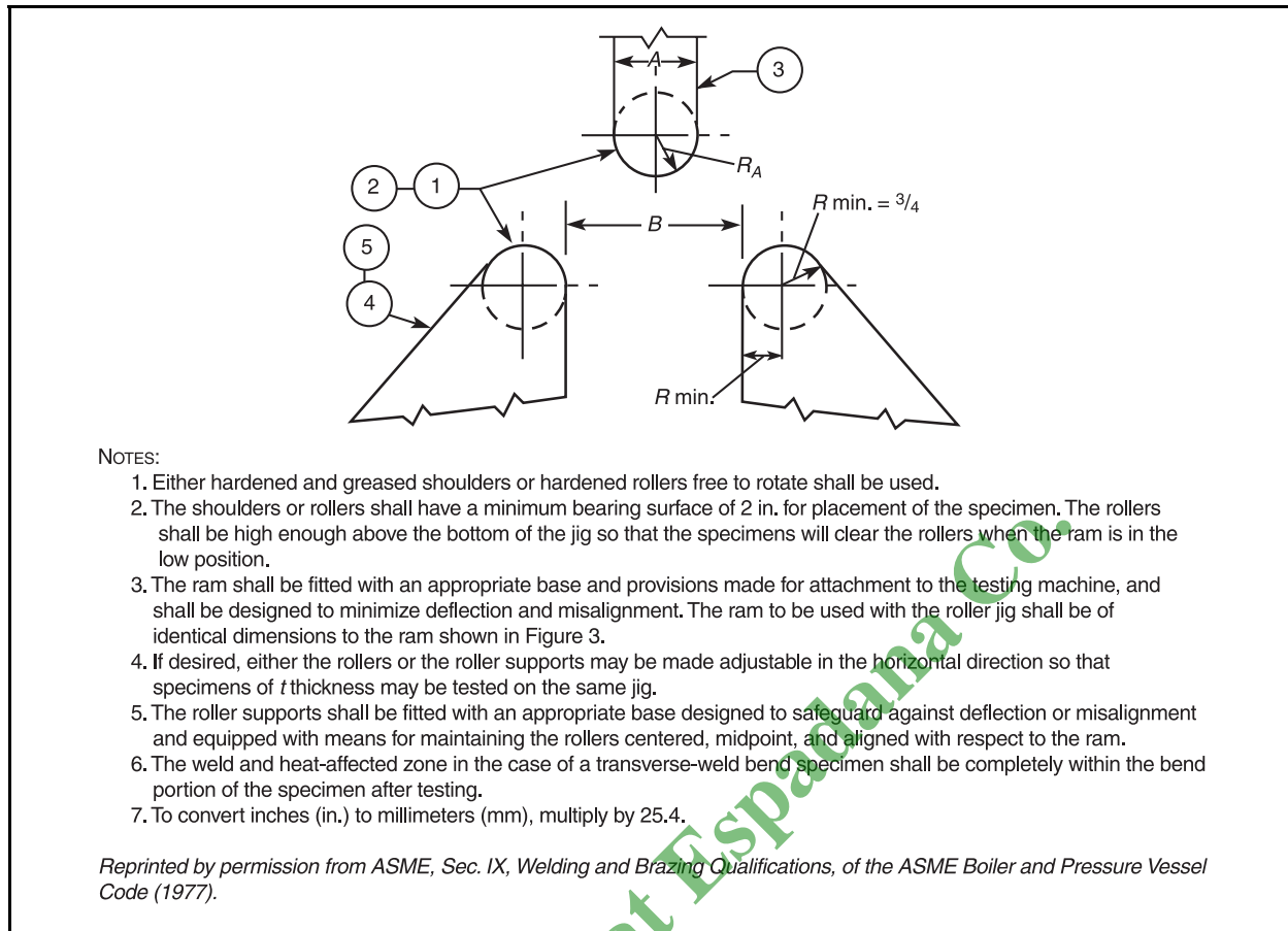
Figure 5 Alternative guided-bend roller jig
